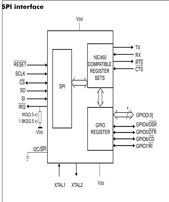
SPI interface
