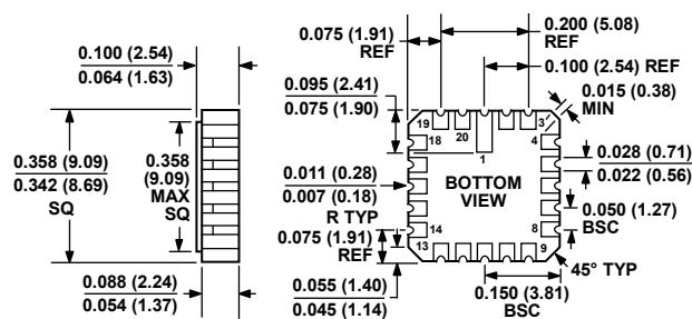
Figure 59. 20-Terminal Ceramic Leadless Chip Carrier [LCC] (E-20-1) RC-Suffix
