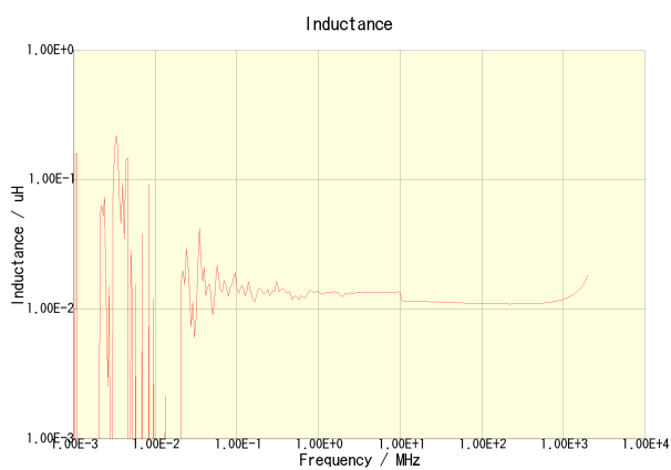
NLV32T-010J-PF
