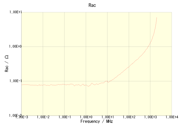
NLV32T-010J-PF
