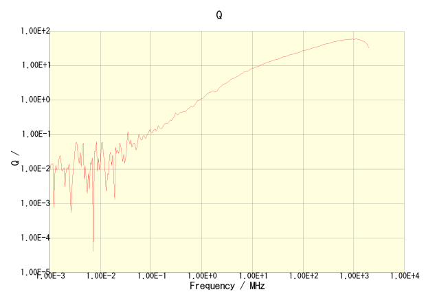
NLV32T-010J-PF
