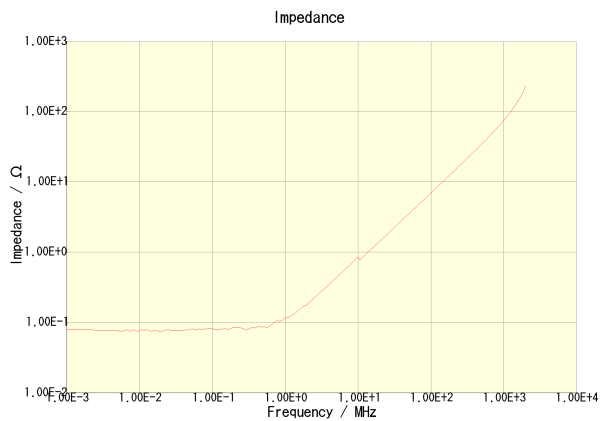
NLV32T-010J-PF
