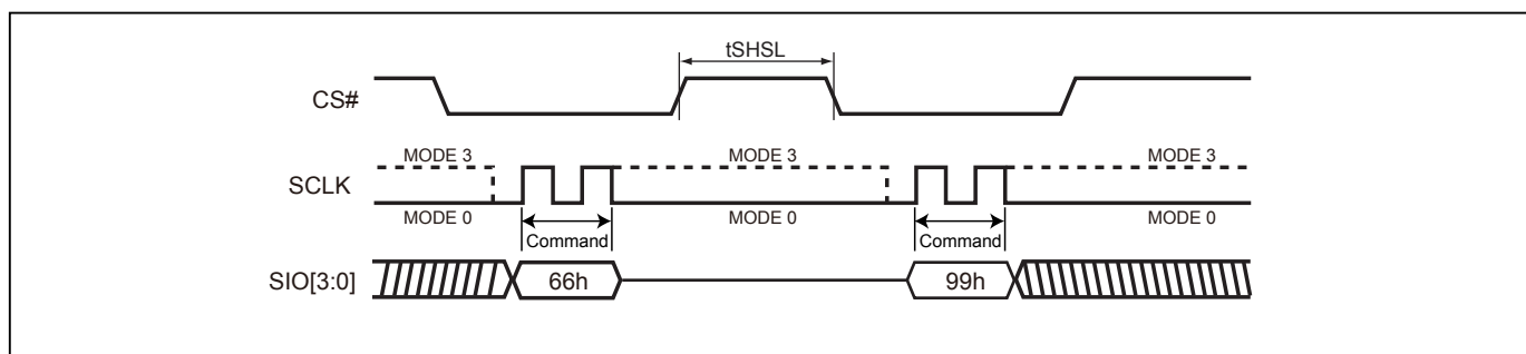
Figure 89. Reset Sequence (QPI mode)
