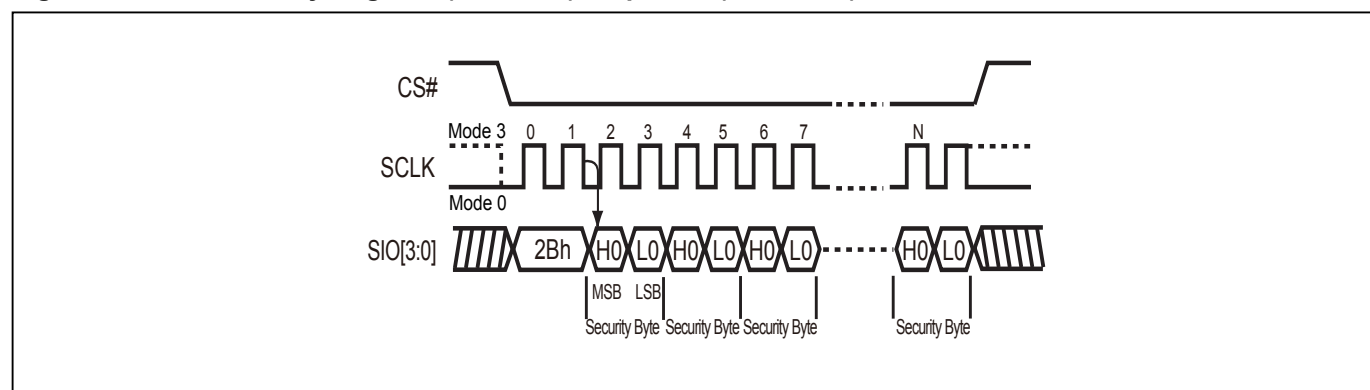
Figure 73. Read Security Register (RDSCUR) Sequence (QPI Mode)
