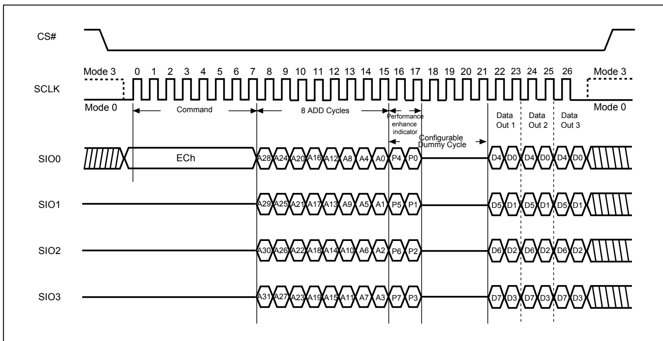
Figure 50. 4 I/O Fast Read using 4-Byte Address sequence (4READ4B)
