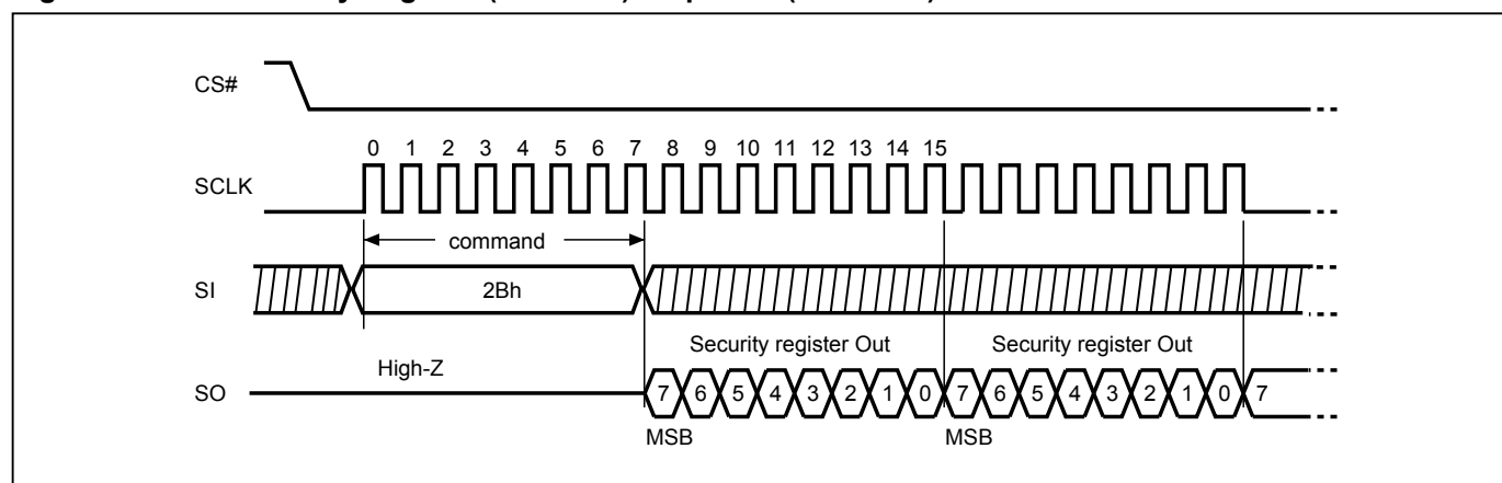
Figure 72. Read Security Register (RDSCUR) Sequence (SPI Mode)
