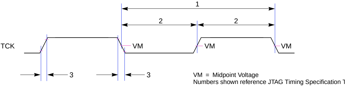
Figure 45. Timing Diagram — JTAG Clock Input
