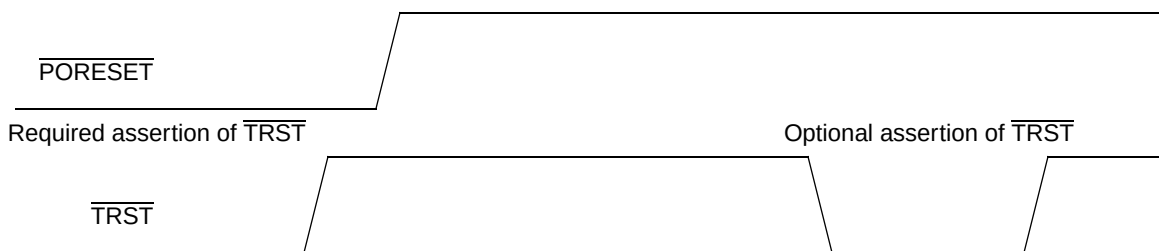
Figure 50. PORESET vs. TRST
