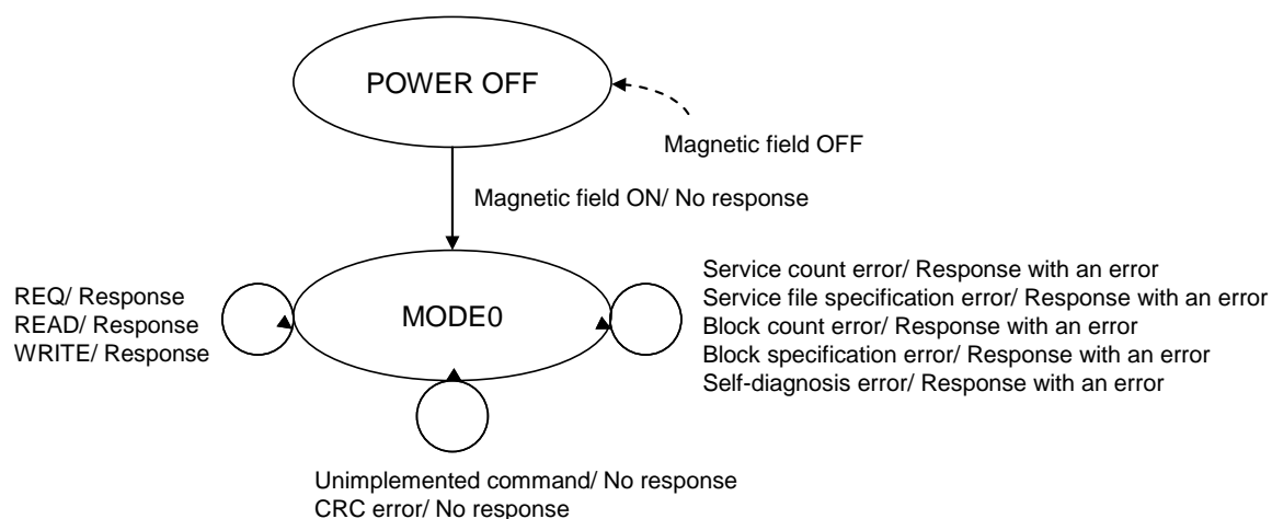
Figure 4-3 State Transition Diagram of JISX6319-4 PICC
