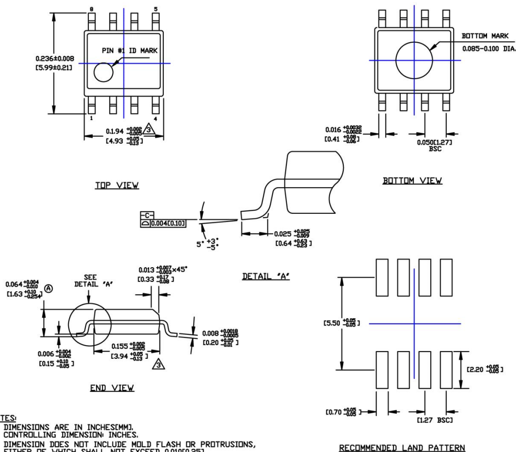
8-Pin SOIC (M)
