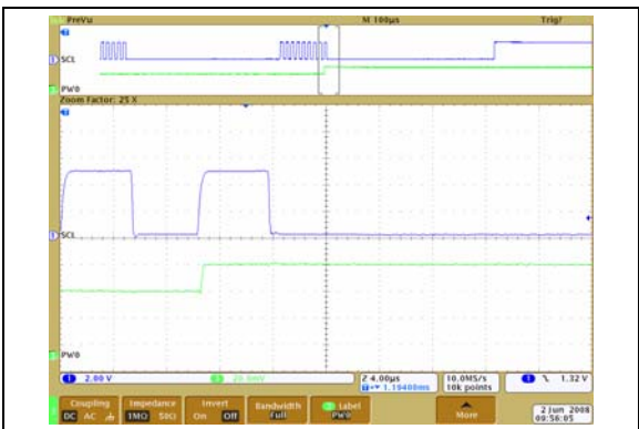
FIGURE 2-15: 5 k \Omega – Low-Voltage Increment Wiper Settling Time ( V_{DD} = 5.5V ) (1 \mu s/Div ).
