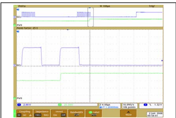
FIGURE 2-16: 5 k \Omega – Low-Voltage Increment Wiper Settling Time ( V_{DD} = 2.7V ) (1 \mu s/Div ).
