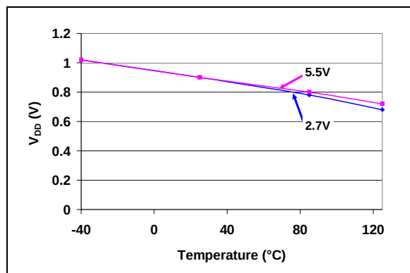
FIGURE 2-57: POR/BOR Trip Point vs. V_{DD} and Temperature.
