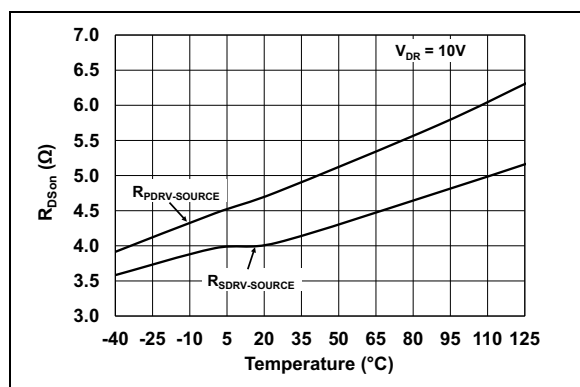
FIGURE 7-8: Sourcing Output Driver R_{DSon} vs. Temperature.
