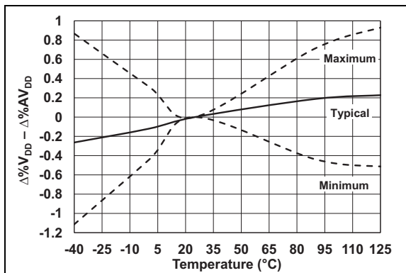
FIGURE 7-15: V_{DD} vs. \Delta V_{DD} Temperature Drift Tracking.
