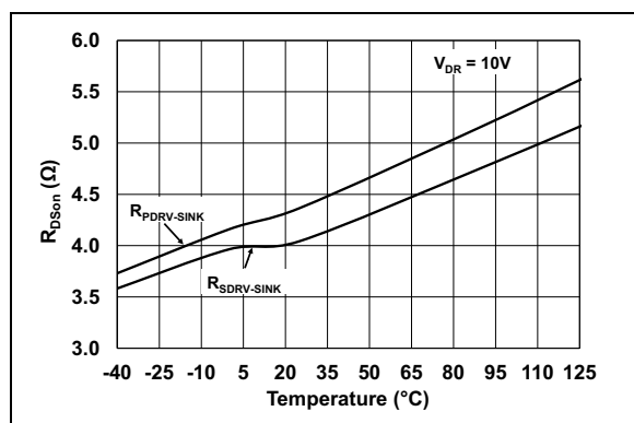
FIGURE 7-9: Sinking Output Driver R_{DSon} vs. Temperature.
