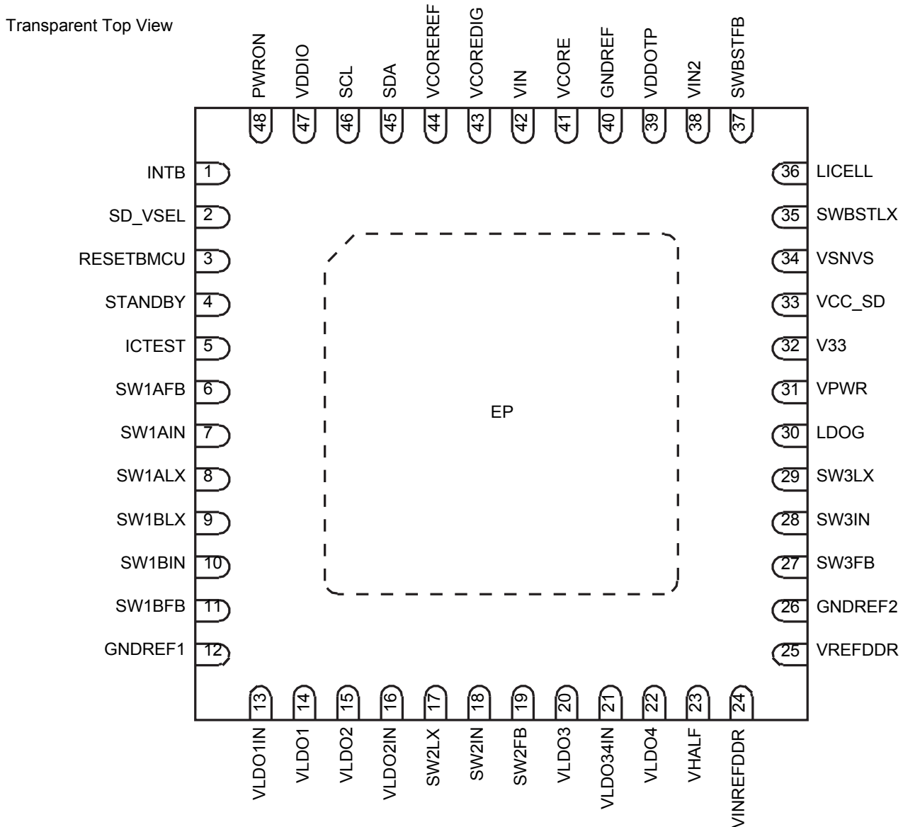
Figure 4. Pinout diagram
