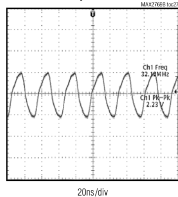
CLOCK OUTPUT DRIVER WITH 40pF LOAD
