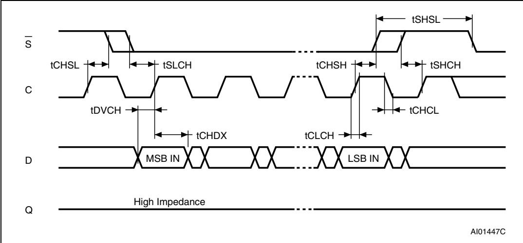
Figure 21. Hold timing
