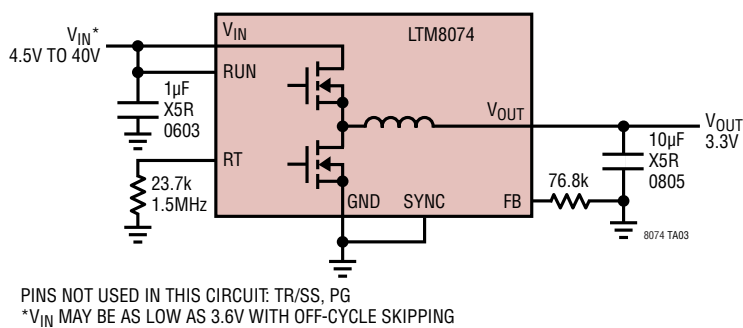
3.3V OUT from 4.5V IN to 40V IN Step-Down Converter
