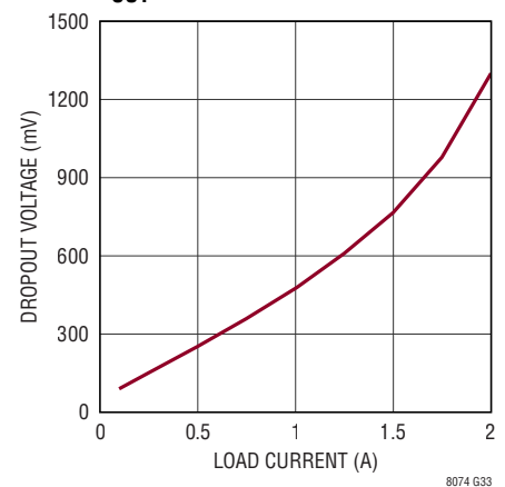
Dropout Voltage vs Load Current V_{OUT} = 5\text{V} , BIAS = 5V
