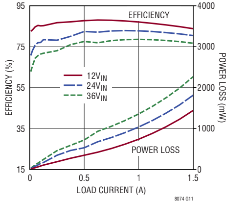
Efficiency and Power Loss, V_{OUT} = 5V , f_{SW} = 2MHz
