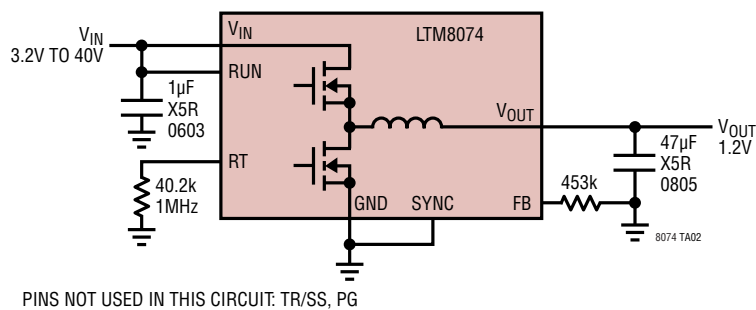
1.2V OUT from 3.2V IN to 40V IN Step-Down Converter
