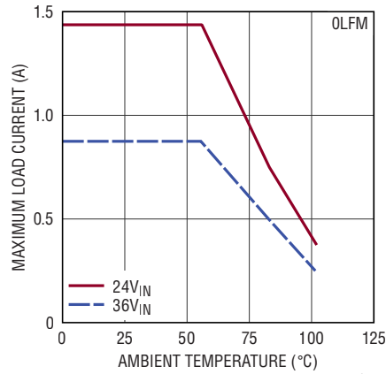
Derating, V_{OUT} = 12\text{V} , DC2753A Demo Board
