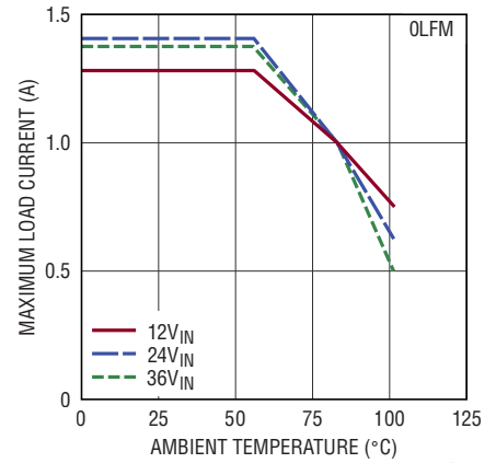
Derating, V_{OUT} = -3.3\text{V} , DC2753A Demo Board
