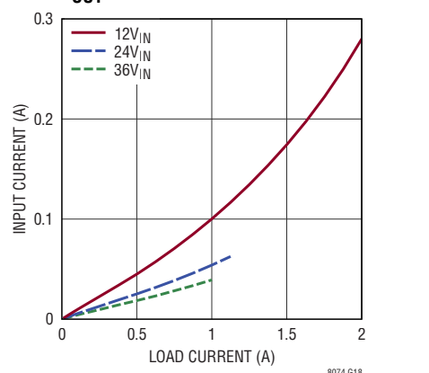
Input vs Load Current, V_{OUT} = 0.8V
