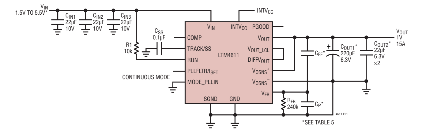
Figure 21. 1.5V to 5.5V IN , 1V at 15A Design
