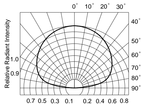
FIG.6 RADIATION DIAGRAM
