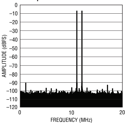
LTC2171-14: 8k Point 2-Tone FFT, f_{IN} = 68\text{MHz} , 69\text{MHz} , -1\text{dBFS} , 40\text{Mpsps}
