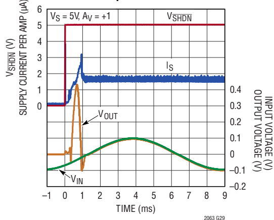
Enable Transient with Sinusoidal Input
