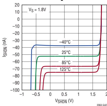
\overline{SHDN} Pin Pull-Up Current vs \overline{SHDN} Pin Voltage
