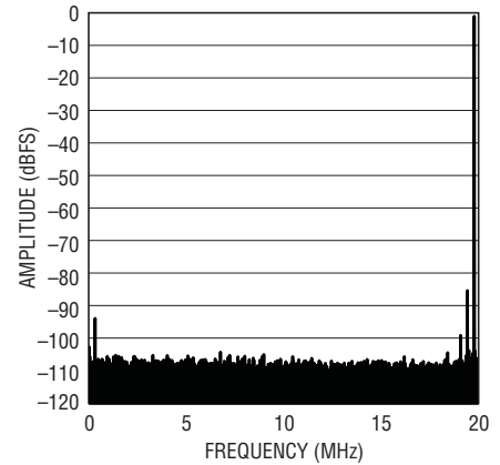
LTC2141-12: 64k Point FFT, f_{IN} = 140\text{MHz} , -1\text{dBFS} , 40\text{MSPS}
