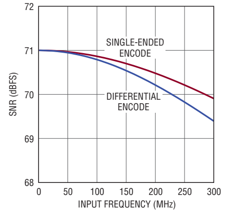
LTC2140-12: SNR vs Input Frequency, -1\text{dBFS} , 25\text{Mps} , 2\text{V} Range
