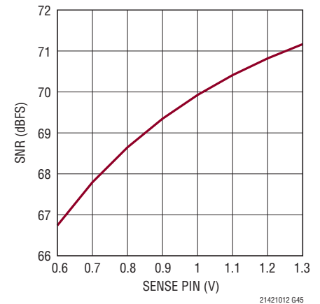
LTC2140-12: SNR vs SENSE, f_{IN} = 5\text{MHz} , -1\text{dBFS}
