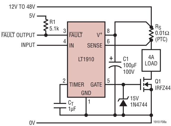
Figure 8a. Low Side Driver with Load Current Sensing
