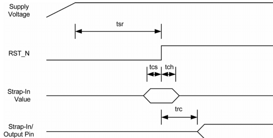
Figure 31. Reset Timing
