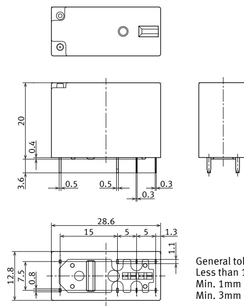
External dimensions
