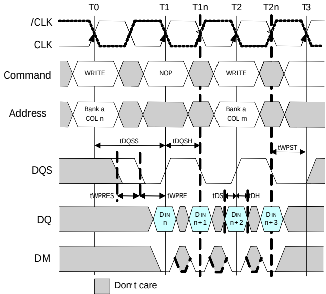
Figure21 : Write Burst (BL=4)
