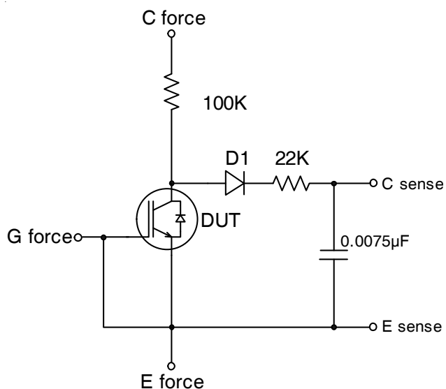
Fig.C.T.6 - BVCS Filter Circuit
