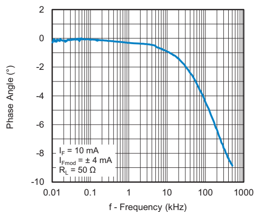
Fig. 8 - Phase Angle vs. Frequency
