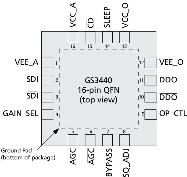
Figure 1-1: GS3440 Pin Out
