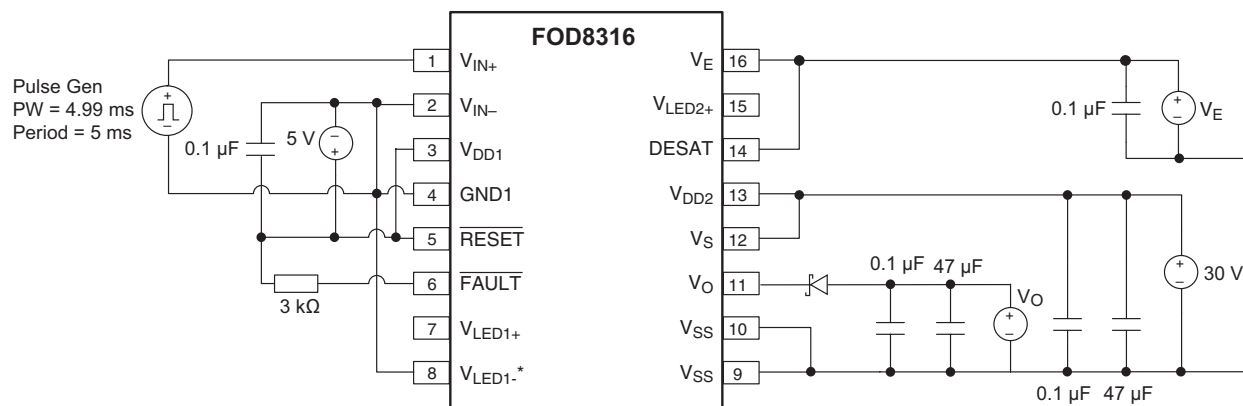
Figure 35. High Level Output Current ( I_{\text{OH}} ) Test Circuit
