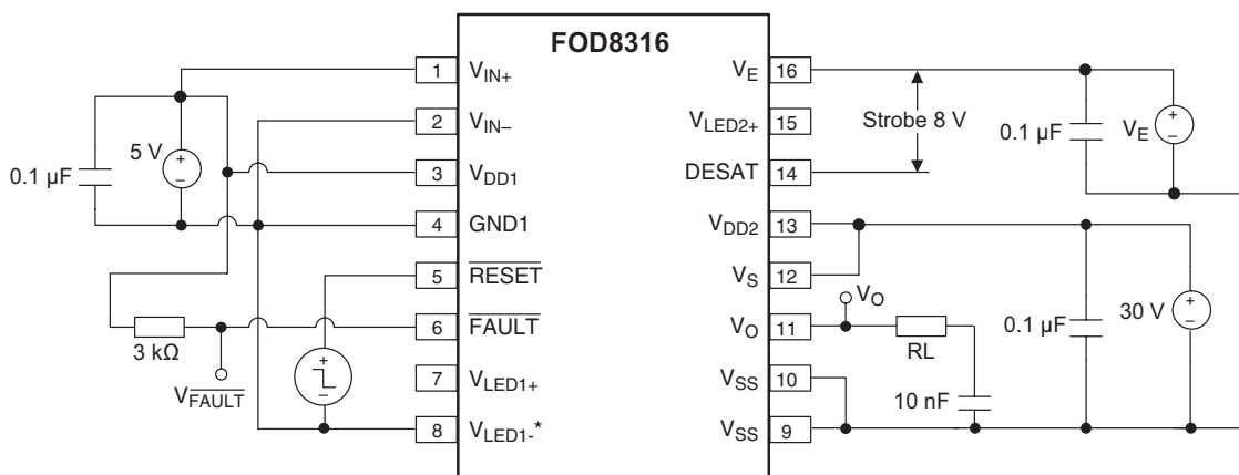
Figure 43. DESAT Sense ( t_{\text{DESAT}(90\%)} , t_{\text{DESAT}(10\%)} ), DESAT Fault ( t_{\text{DESAT}(\text{FAULT})} ), and ( t_{\text{DESAT}(\text{LOW})} ) Test Circuit
