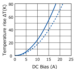
[ ETQP4M1R5KVK ]
