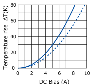
[ ETQP4M6R8KVK ]
