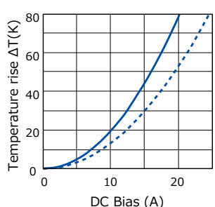
[ ETQP4M1R5KVC ]
