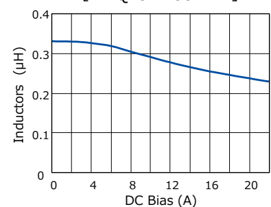
[ ETQP3MR33KVP ]
