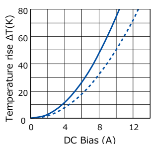
[ ETQP4M6R8KVC ]
