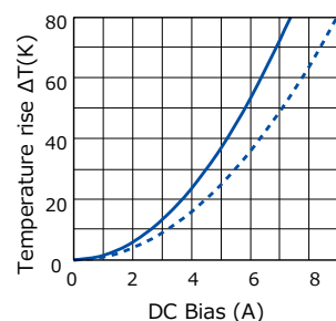
[ ETQP4M150KVC ]
