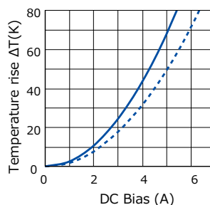
[ ETQP4M150KVK ]
