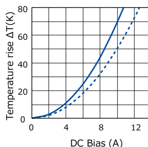
[ ETQP4M3R3KVK ]
