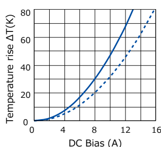
[ ▲ETQP4M4R7KVC ]
