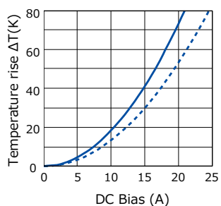
[ ETQP4M1R0KVK ]
