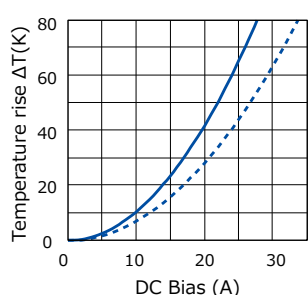
[ ETQP4M1R0KVC ]
