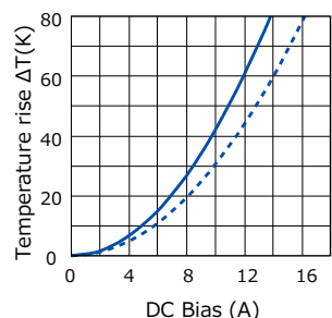
[ ETQP4M2R2KVK ]
