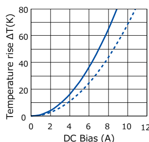
[ ETQP4M100KVC ]
