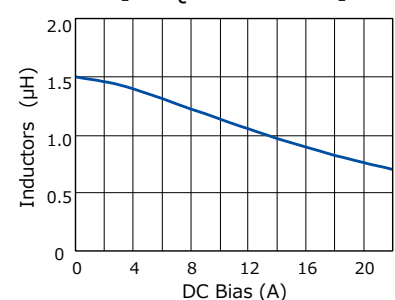
[ ETQP3MR33KVP ]
