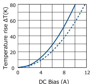
[ ETQP4M4R7KVK ]
