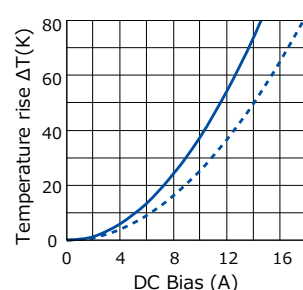
[ ETQP4M3R3KVC ]
