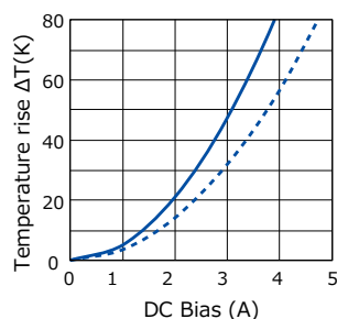
[ ETQP4M470KVC ]
