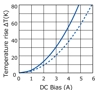
[ ETQP4M330KVC ]
