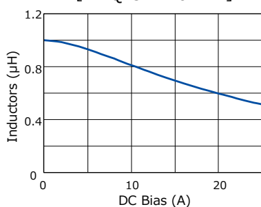
[ ETQP3M1R0KVP ]
