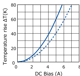
[ ETQP4M220KVC ]
