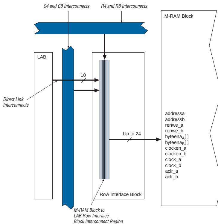
Figure 4–21. M-RAM Row Unit Interface to Interconnect
