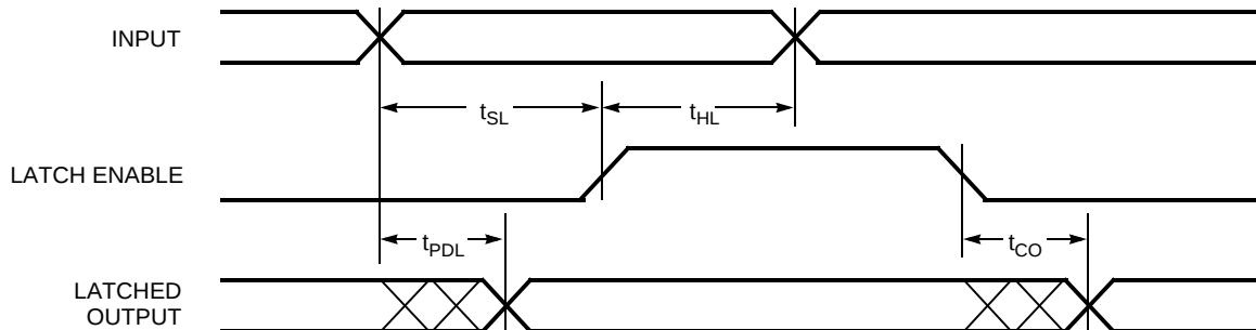
Figure 13. Latched Output
