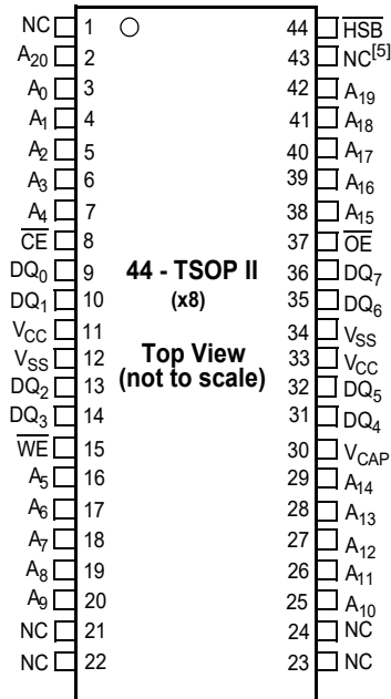
Figure 1. Pin Diagram: 44-Pin TSOP II (×8)
