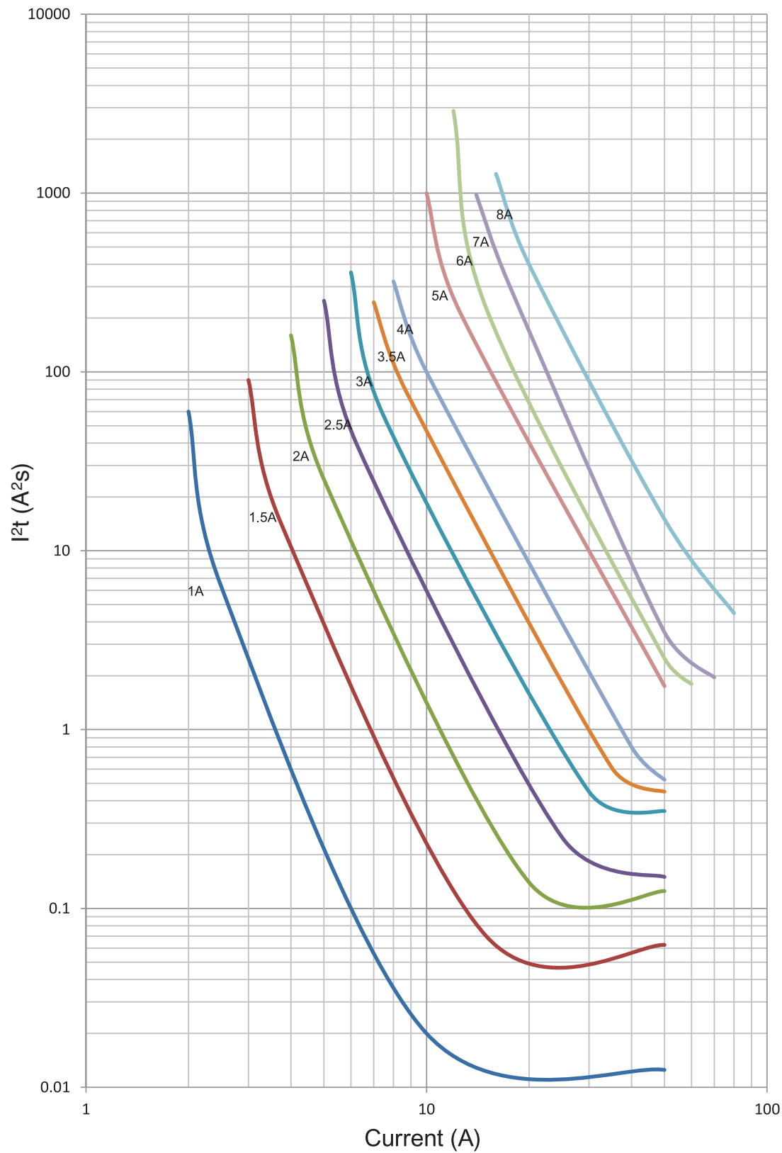
I 2 t vs. current curves
