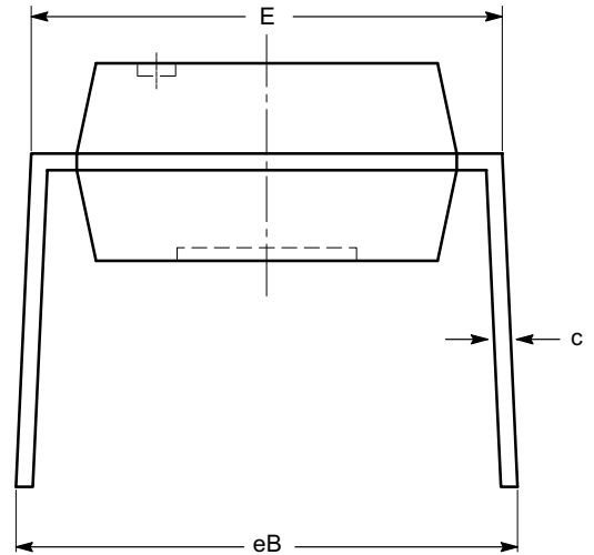
END VIEW
