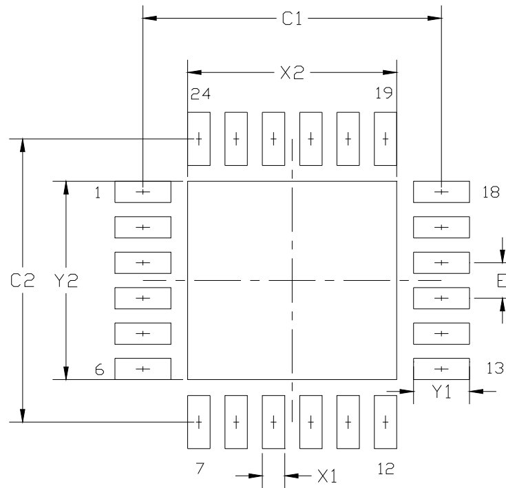
Figure 4.9. Typical QFN-24 Landing Diagram
