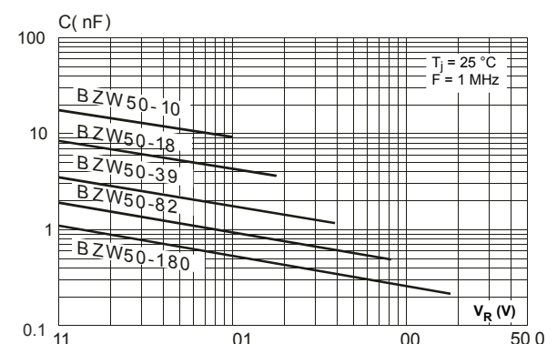
Figure 6. Capacitance vs. reverse applied voltage for unidirectional types (typical values)
