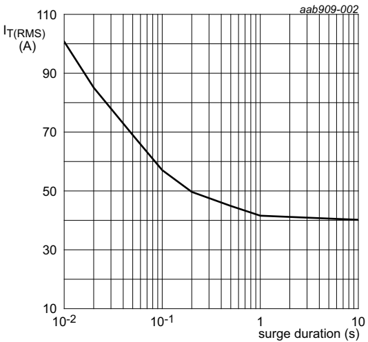
f = 50\text{ Hz} ; T_{\text{mb}} = 110\text{ }^{\circ}\text{C} Fig. 2. RMS on-state current as a function of surge duration; maximum values
