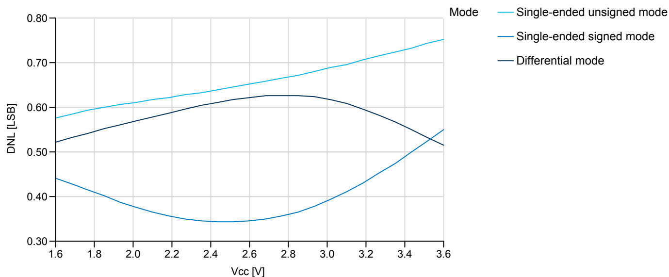
Figure 37-49.DNL Error vs. V_{CC} T = 25^{\circ}\text{C} , V_{REF} = 1.0\text{V}
