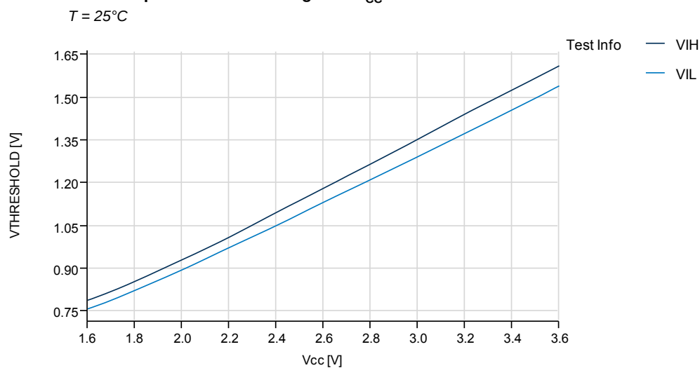
Figure 37-34. I/O Pin Input Threshold Voltage vs. V_{CC}
