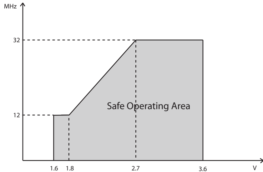
Figure 34-1. Operating Frequency vs.Vcc
