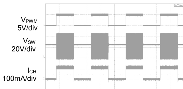
PWM Dimming
