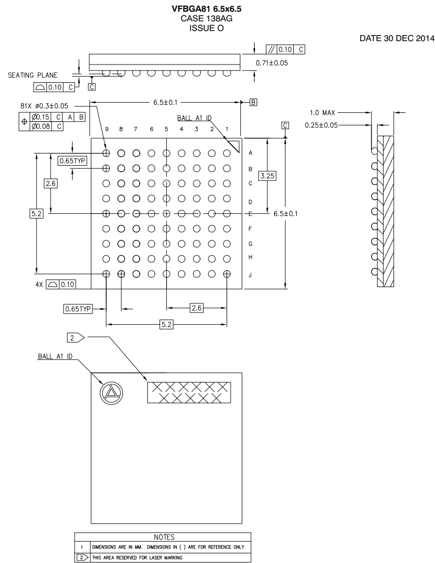
Figure 29: Package Diagram
