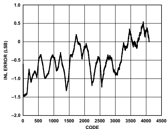
Figure 22. DAC INL Error vs. Code
