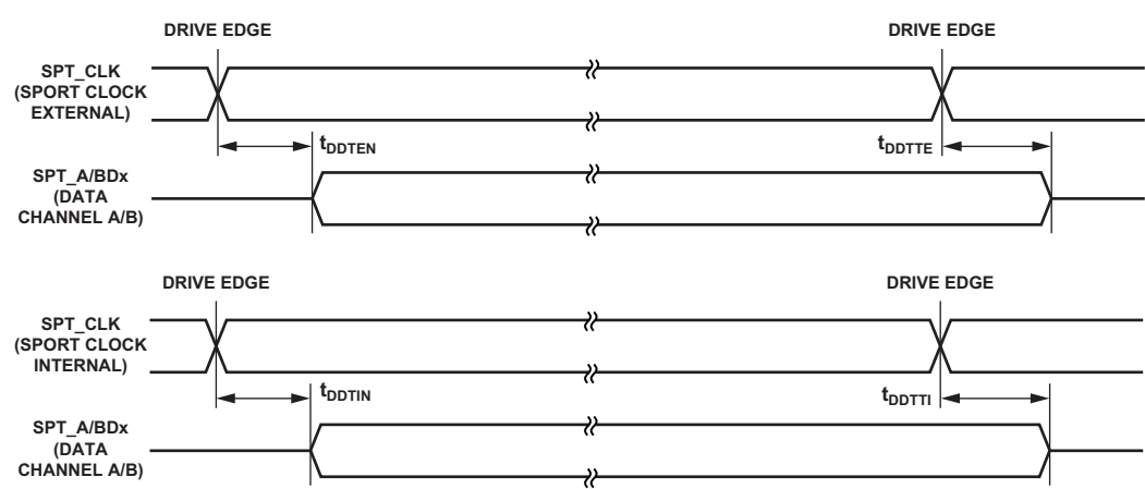
Figure 32. Serial Ports—Enable and Three-State
