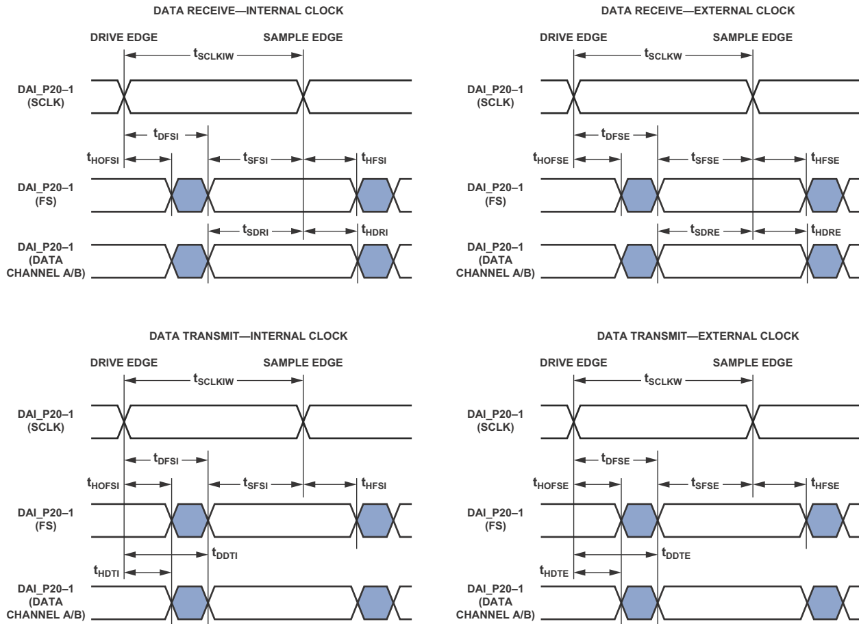
Figure 26. Serial Ports
