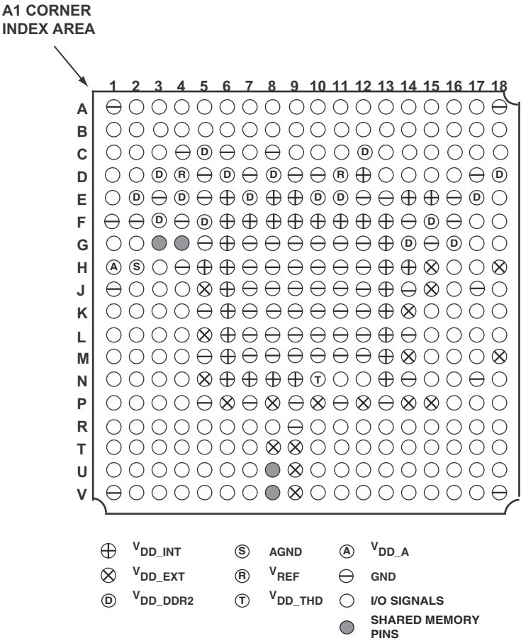
Figure 60. Ball Configuration, Automotive Model
