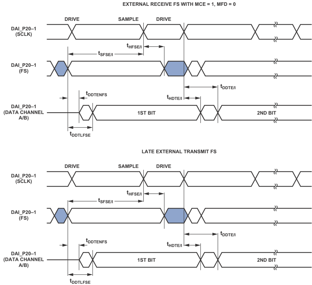
Figure 29. External Late Frame Sync
