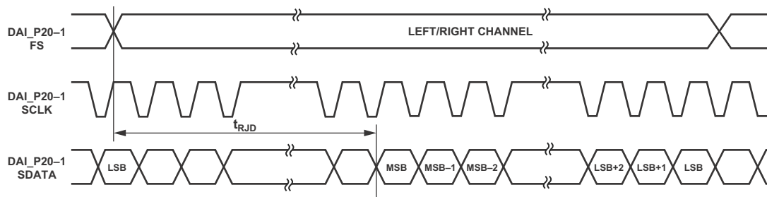
Figure 35. Right-Justified Mode
