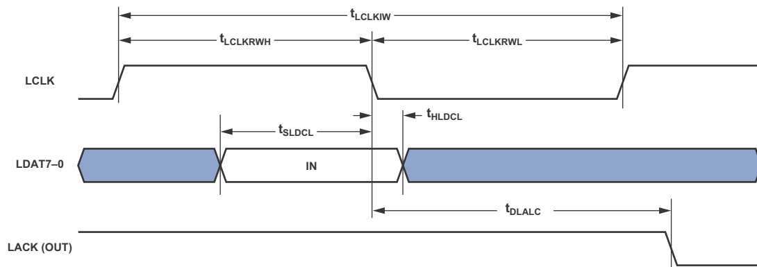
Figure 23. Link Ports—Receive
