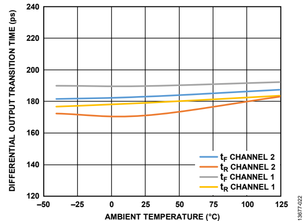
Figure 26. Differential Output Transition Time vs. Ambient Temperature ( T_A )
