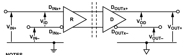
Figure 36. Voltage Definitions
