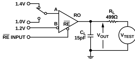
Figure 30. Receiver Timing Measurement
