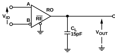
Figure 30. Receiver Timing Measurement
