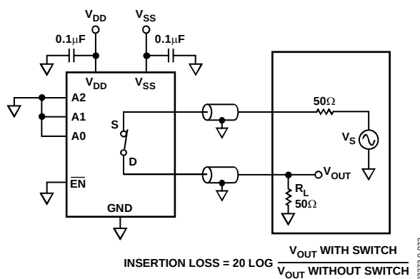
Figure 30. Bandwidth
