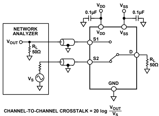
Figure 29. Channel-to-Channel Crosstalk
