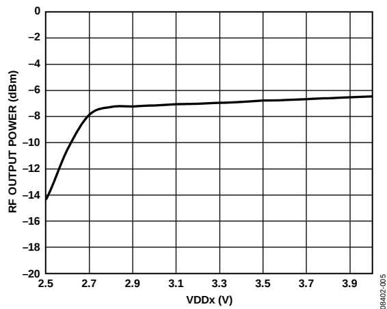
Figure 5. RFOUT Power (Single-Ended) vs. VDDx, f_{IN} = 10 GHz, P_{IN} = 0 dBm
