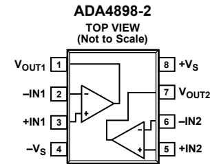
Figure 6. Dual 8-Lead SOIC_N_EP Pin Configuration
