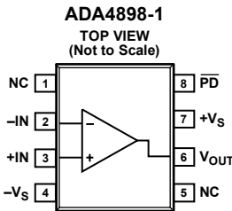
Figure 5. Single 8-Lead SOIC_N_EP Pin Configuration
