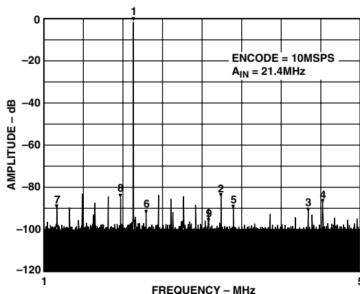
Figure 33. IF Sampling a 21.4 MHz Input Using the AD9220 ( V_{CM} = 2.5 \text{ V} , Input Span = 2 \text{ V p-p} )
