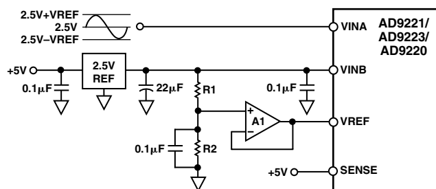
Figure 24. External Reference— V_{CM} = 2.5\text{ V} (2.5 V on VINB, Resistor Divider to Make VREF)
