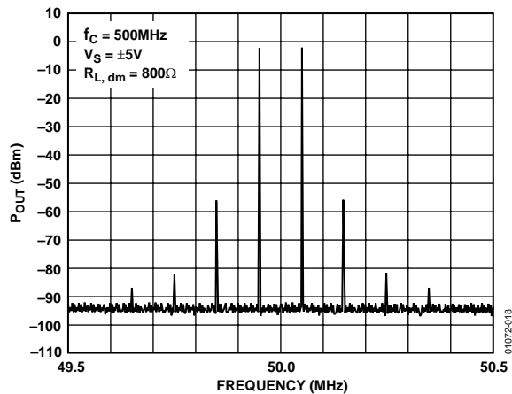
Figure 19. Intermodulation Distortion
