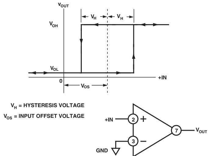
Figure 6. Hysteresis Definitions (N, Q Package Pinout)
